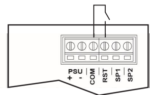
Reset for Peak Hold
