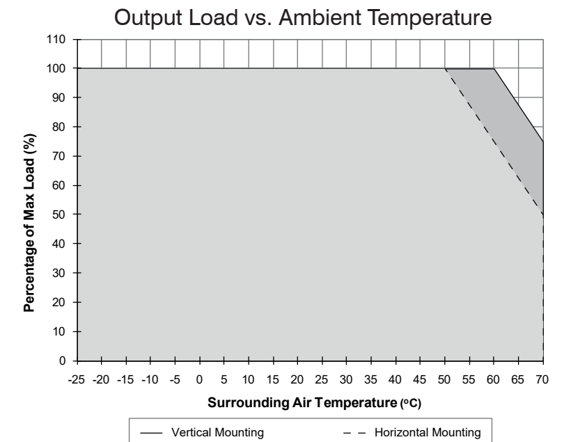
RHINO PRO PSD24-120-L Temperature Derating Curve
