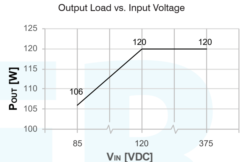
RHINO TOUGH PSX-24-120 Input De-rating Curve
