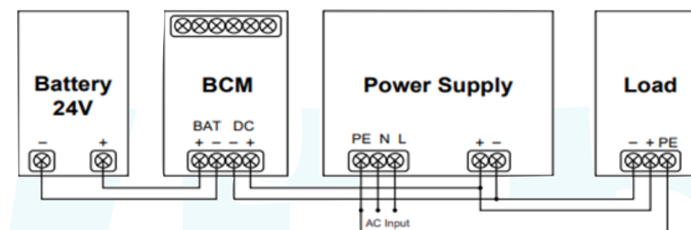
Battery Control Module wiring diagram
