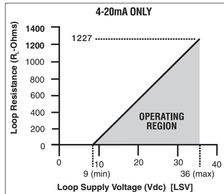
Power Supply Voltage vs Loop Resistance
