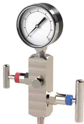
Example assembly of BBV series block and bleed valve and G25 series pressure gauge.
