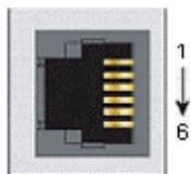
6-pin RJ12 Female Modular Connector
