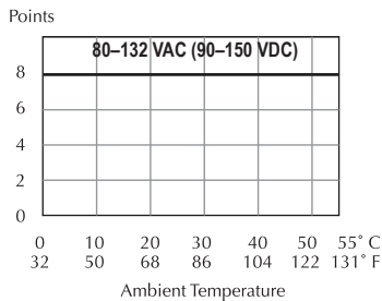
Derating chart
