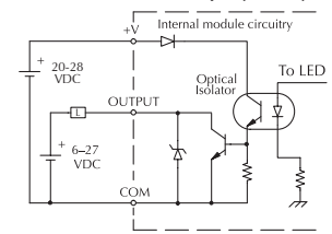
Equivalent output circuit Standard output (Y2-Y17)
