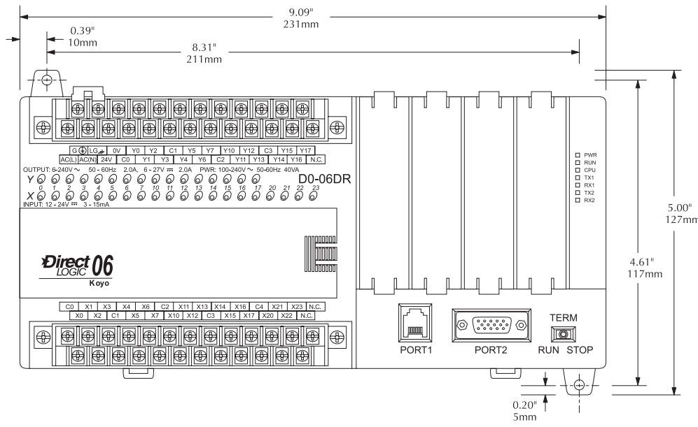
Mounting orientation
