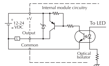
Equivalent output circuit Standard output (Y2-Y17)
