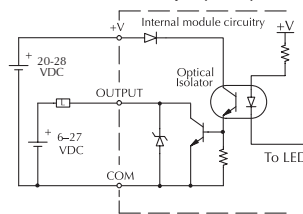
Equivalent output circuit Pulse output (Y0-Y1)
