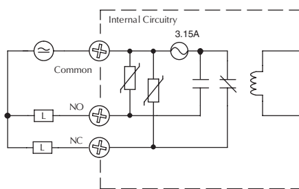
Typical Circuit
