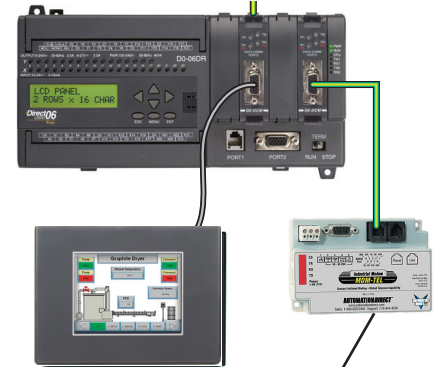
DL06 PLC with multiple DCM modules
