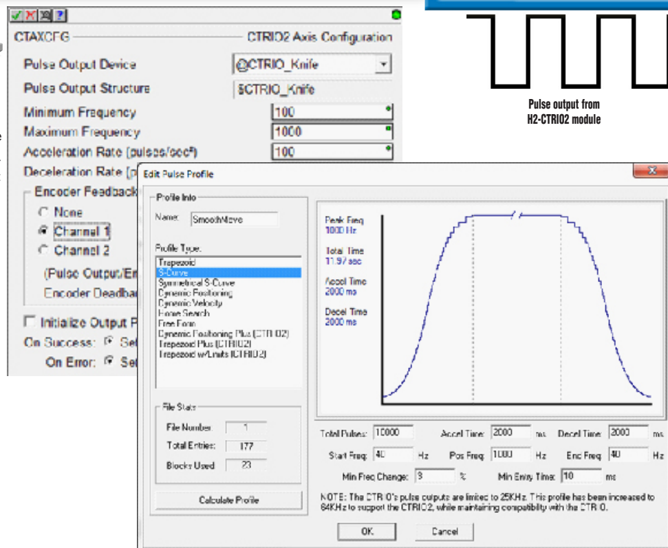
AutomationDirect Do-more PLC with H2-CTRIO2 modules ($445,000) using pulse output feature
