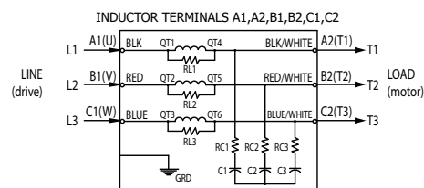
INDUCTOR AND BOARD ASSEMBLY CONNECTIONS
