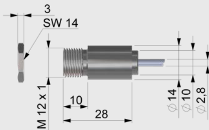
Dimensions CSmicro
