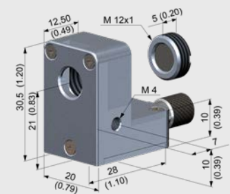
Air purge with integrated CF optics (ACCTAPLCF)
