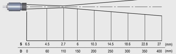
CF optics, D:S = 40:1
