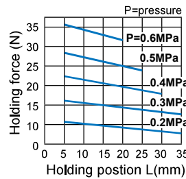
MCHG2-25
