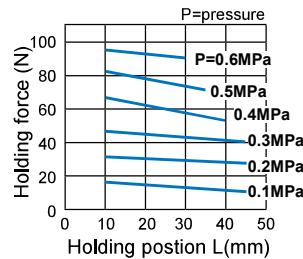
MCHG2-40
