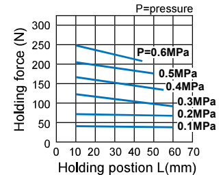
MCHG2-63
