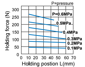
MCHG2-63
