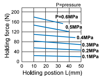
MCHG2-40
