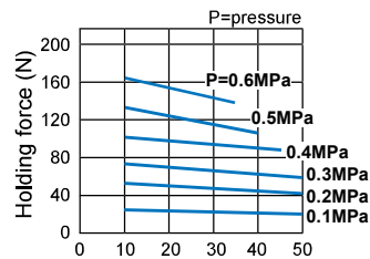
MCHG2-40
