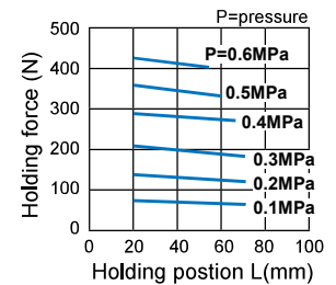
MCHG2-80
