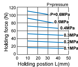
MCHG2-40
