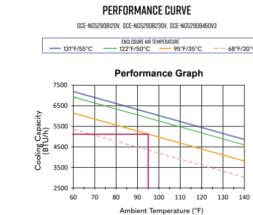
The NEMA 12 460VAC selection from this series is SCE-NG5290B460V3 .
