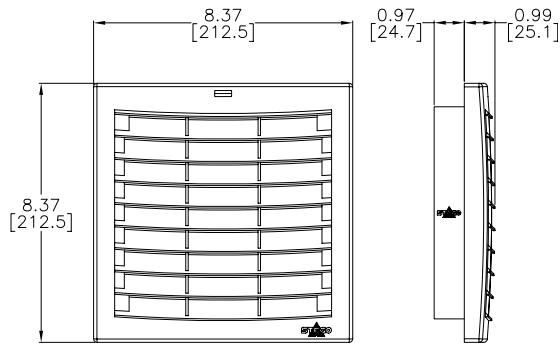
Intake grille for 6.93 x 6.93 in FPO Fan
