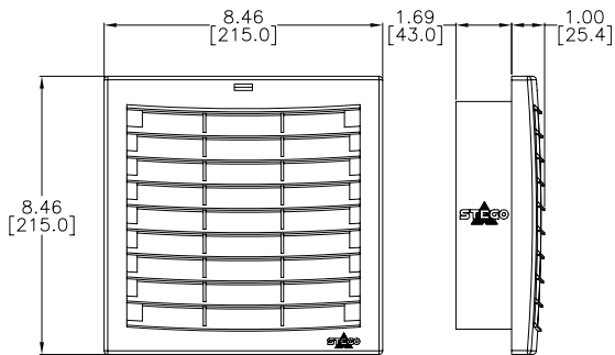
Exhaust grille for 6.93 x 6.93 in FPI Fan
