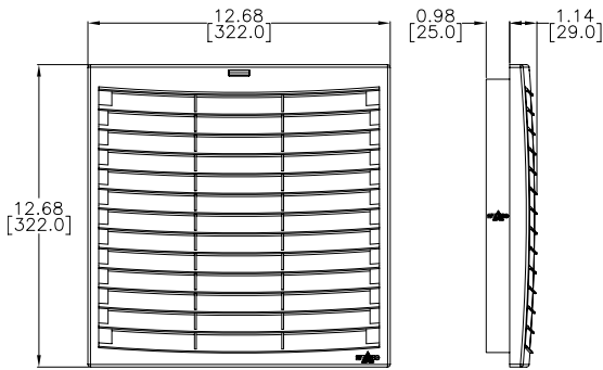
Intake grille for 11.46 x 11.46 in FPO Fan
