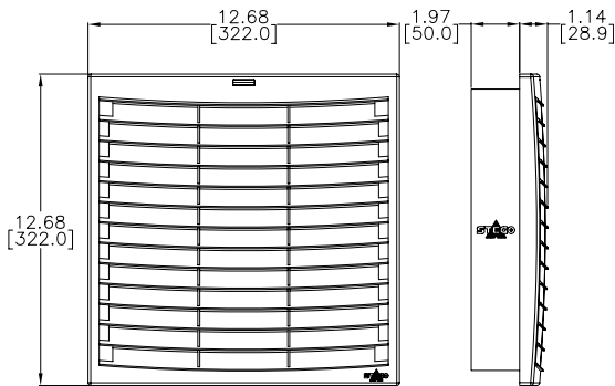
Exhaust grille for 11.46 x 11.46 in FPI Fan
