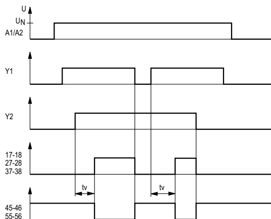
Function Diagram
