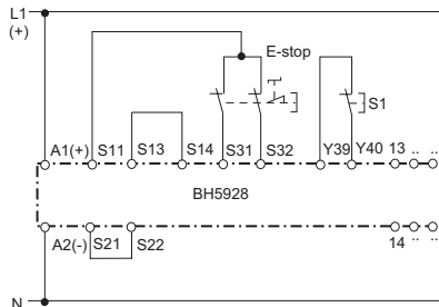
2-channel emergency stop circuit without cross fault monitoring autostart and interruption of time by S1
