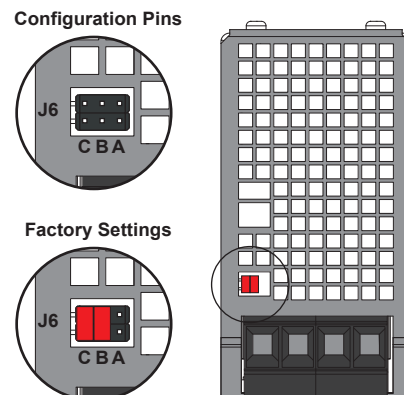
Figure 1 – Configuration Jumpers (Top of Unit)
