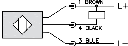
Diagram 3 NPN M8 Connector
