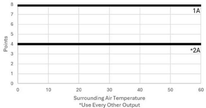
P2-16CDR Output Derating Chart
