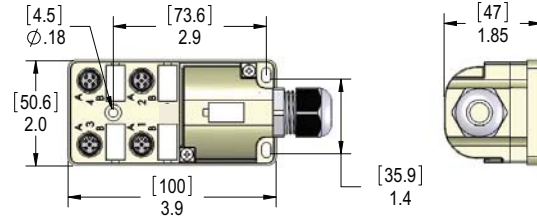
Figure 2: 4 Port 5 Pin
