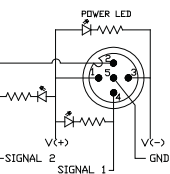
NPN Version Diagram 6-C
