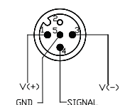
No LED Version Diagram 5-A
