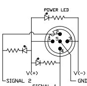
NPN Version Diagram 2-C
