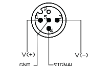
No LED Version Diagram 3-A
