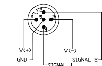
No LED Version Diagram 4-A
