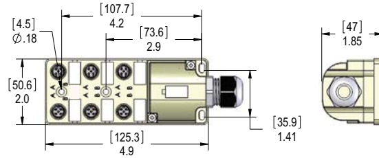
Figure 4: 6 Port 5 Pin
