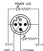
PNP Version Diagram 3-B
