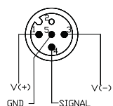
No LED Version Diagram 1-A
