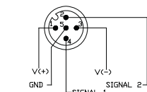
No LED Version Diagram 2-A
