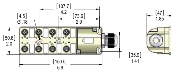
Figure 6: 8 Port 5 Pin
