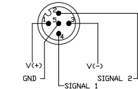
No LED Version Diagram 6-A
