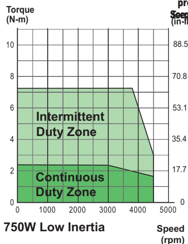
Servo Drive SVA-2100
