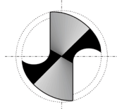
CBN bit with split point DIN 1412C
