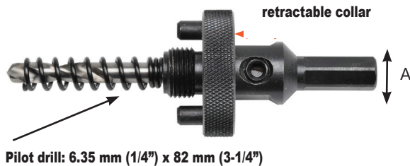
Pilot drill: 6.35 mm (1/4") x 82 mm (3-1/4")
