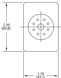
AR-1C-120A, ARX-2C-120A
