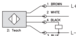
Diagram 2 PNP Output
