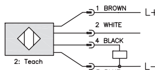
Diagram 2 PNP Output
