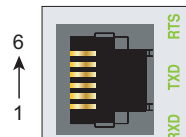
6-pin RJ12 Female Modular Connector
