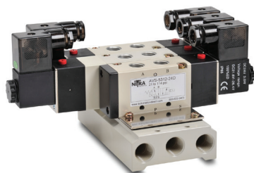
Stacked solenoids shown mounted on optional manifold
