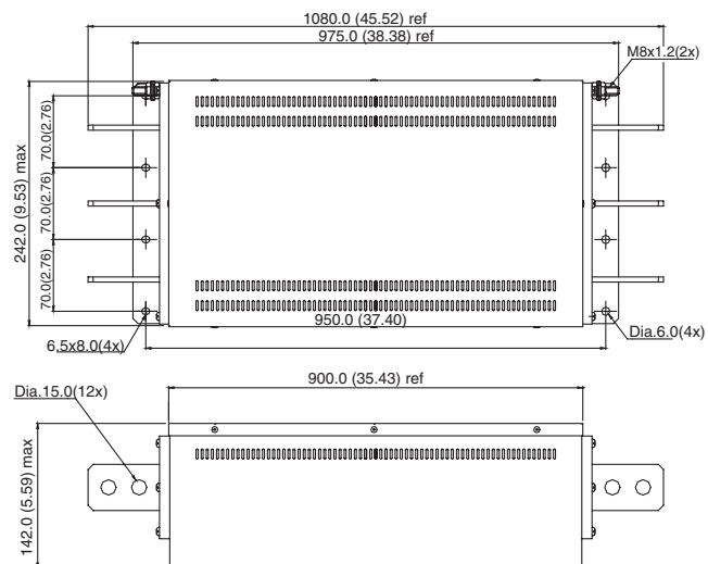
Figure 16 [ units = mm (in) ]
