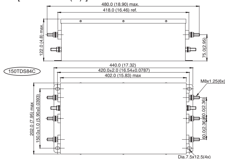
Figure 11 [ units = mm (in) ]
