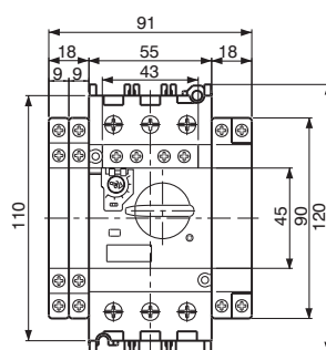
BM3VHB-xxx + BZ0xxxxx
