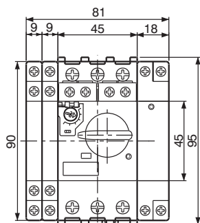
BM3RHB-xxx + BZ0xxxxx
