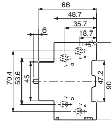
Short-circuit alarm contact block BZ0TKUAB
