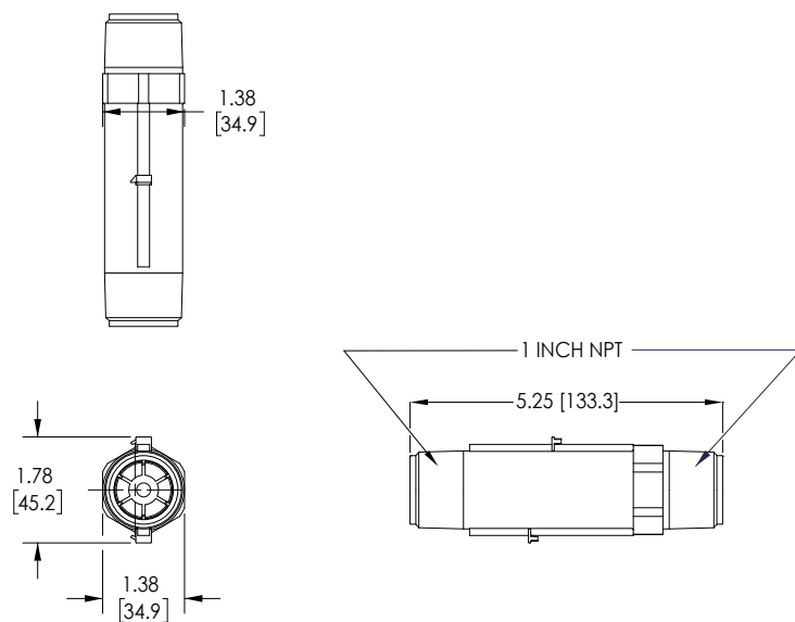
FG1x-100PP-x Models
