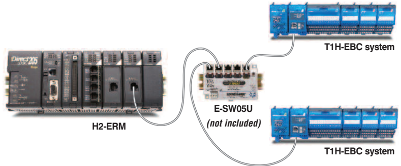
Example of an Ethernet remote I/O system using a T12-ERKIT-2. CPU, bases, I/O modules, Ethernet switch, etc. are sold separately.
