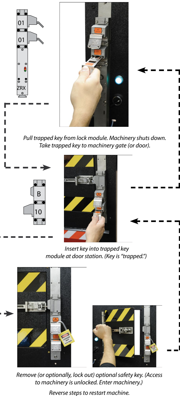
Keys trapped at main station (left). Door station with optional padlock module (right).
