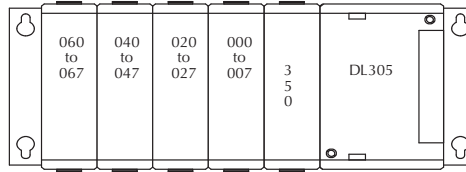
D3-05BDC base using 8-pt. I/O modules
