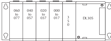
D3-05BDC base using 16-pt. I/O modules
