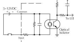
Current sinking configuration shown
