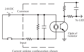
Current sinking configuration shown
