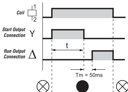
Timing Diagram
