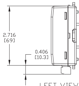
LEFT VIEW
