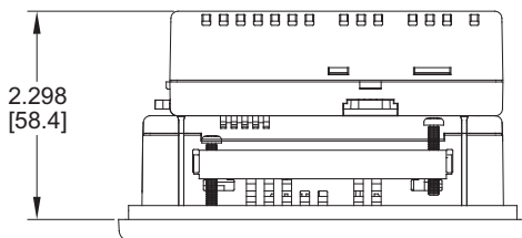
Panel overall depth with adapter installed
