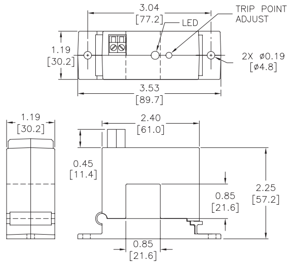
ACSL Series Split Core
