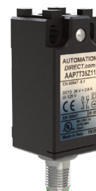
5-pin M12 quick-disconnect (bottom)
