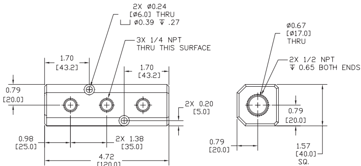
Part No. MLA-3
