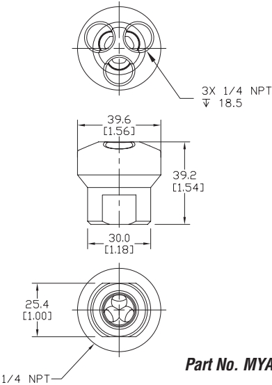
Part No. MYA-2
