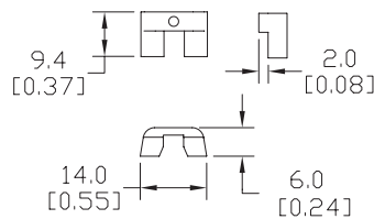
CPS9D-D14M
