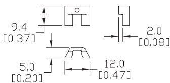
CPS9D-D12M
