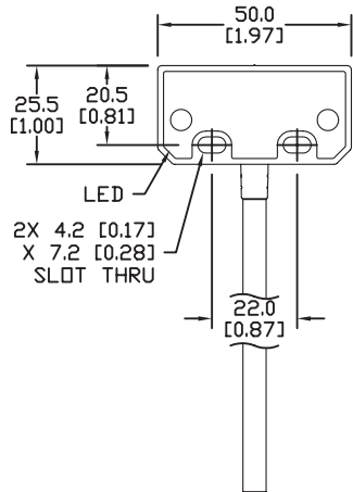
SWITCH
