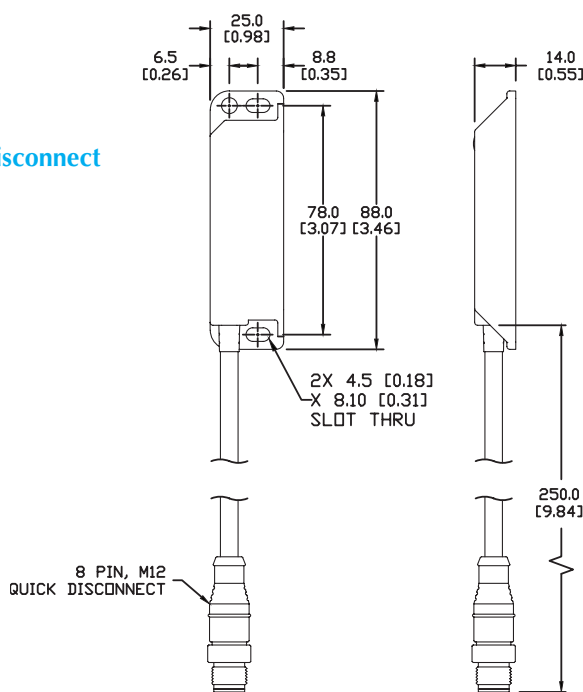
SWITCH
