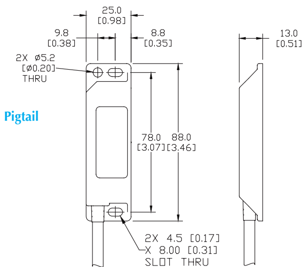
SWITCH
