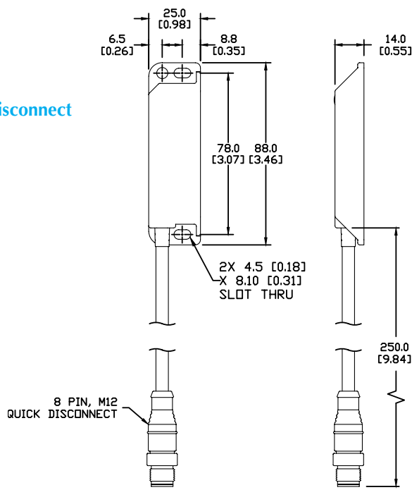
SWITCH
