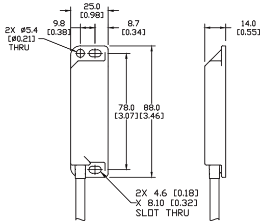
SWITCH
