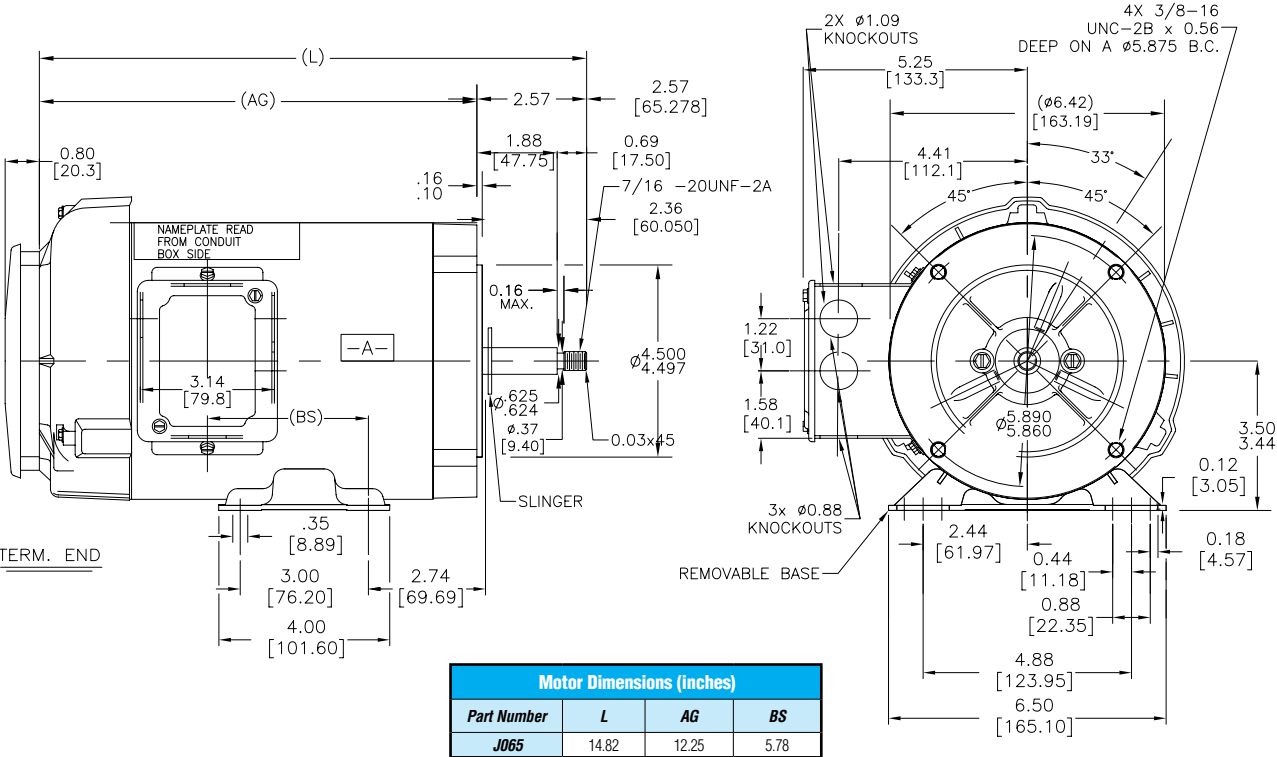
Figure 2 – J065 Dimensions
