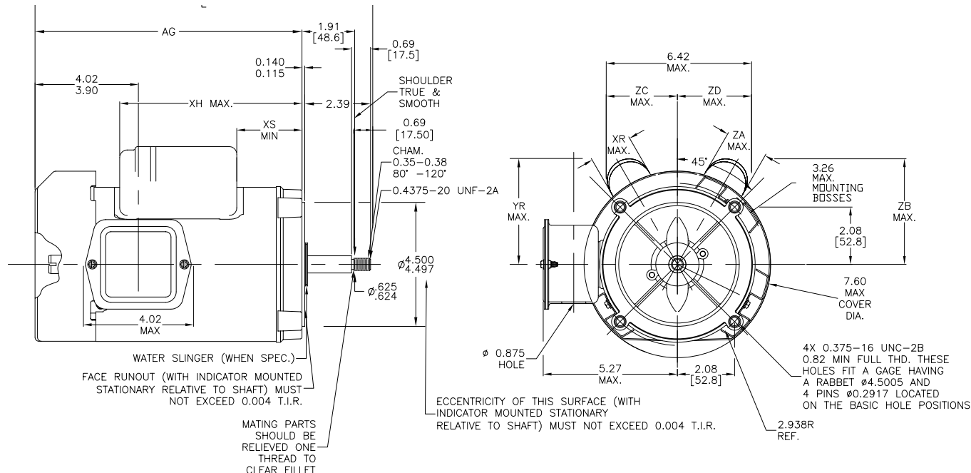
Figure 2 – C878 Dimensions
