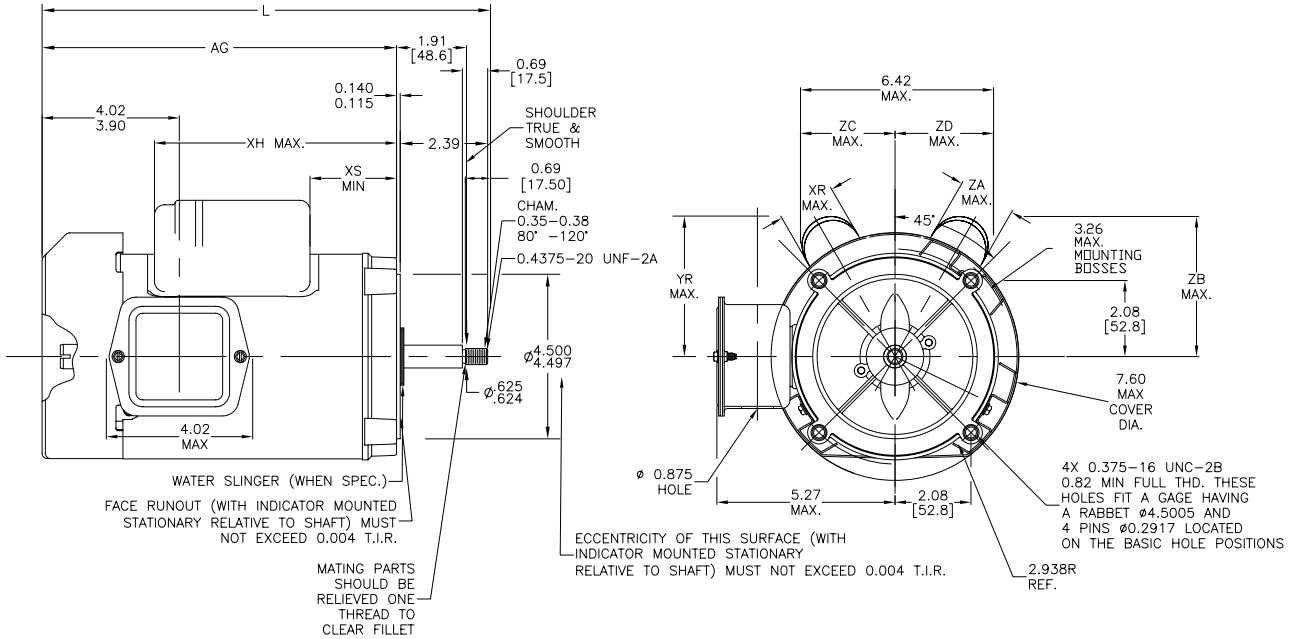
Figure 2 – C878 Dimensions
