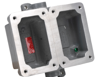
FXB-11 Double Gang Feed Through
