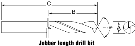
*Point angle for HSS-Co5 bits is 135°
