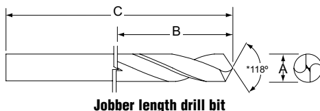
*Point angle for HSS-Co5 bits is 135°
