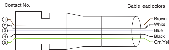
5-pole Connectors
