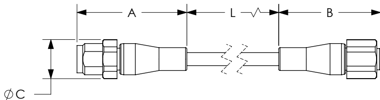
Axial Connectors
