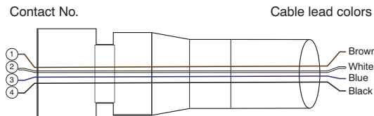
4-pole Connectors
