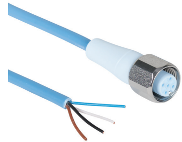
7024-12221-3210200
