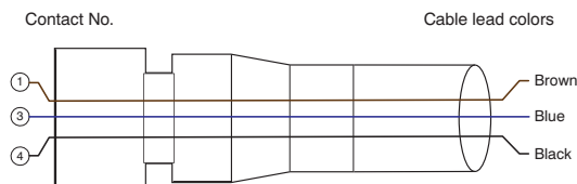
3-pole Connectors
