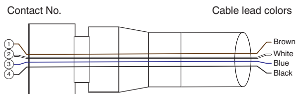
4-pole Connectors
