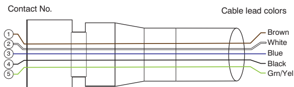
5-pole Connectors
