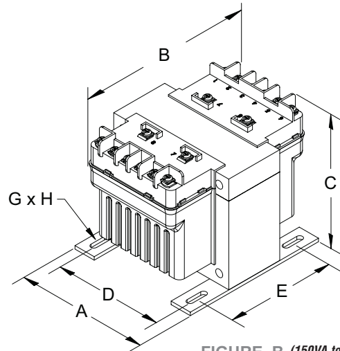
FIGURE B (150VA to 500VA)
