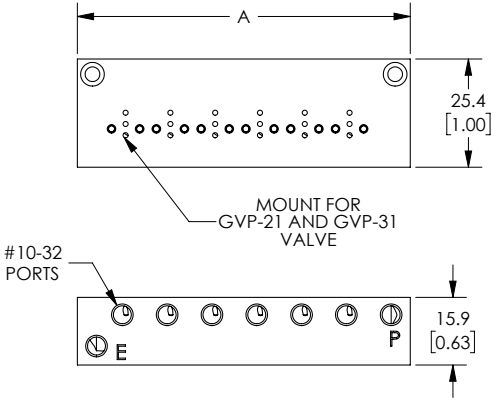
Part No. GM-312, GM-314, GM-316
