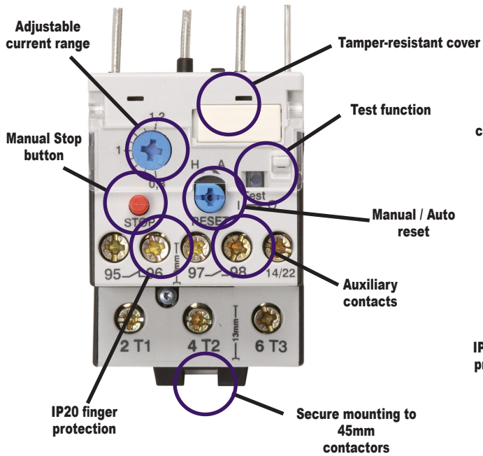
RTD32 for 45mm Contactors
